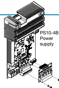
CLA-PS10 Class A Adapter Card
